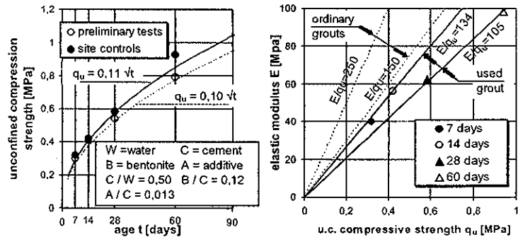
Figure 5. Plastic grouts mechanical properties a) u.c. strength vs. curing time b) E vs. u.c. strength
