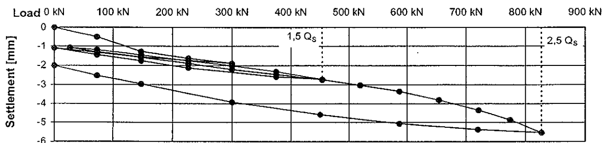
Figure 6. Tubfix micropile - Load test data.
