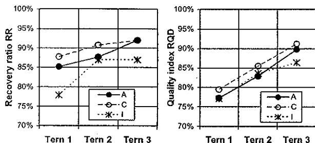
Figure 7. Jet grouting field trial: average core recovery parameters (control boreholes)
