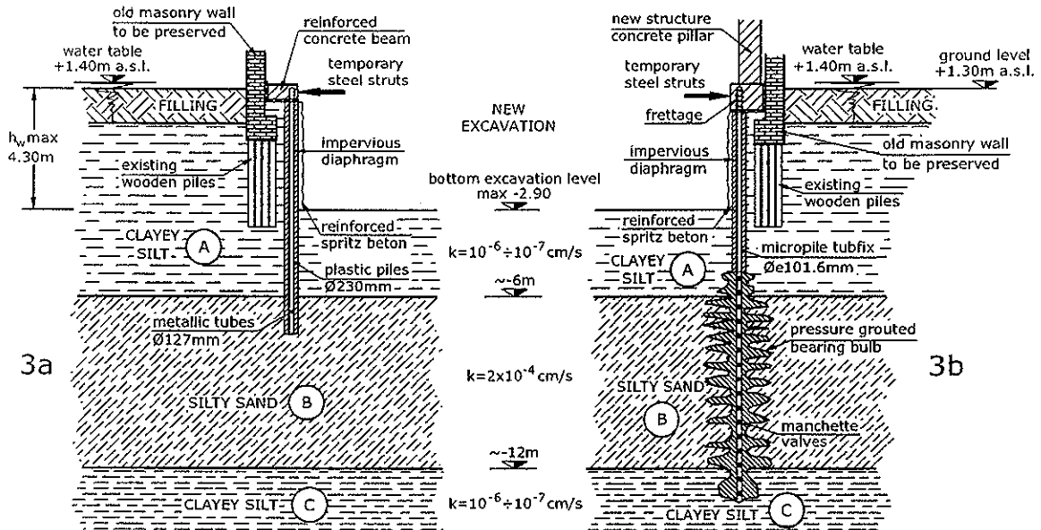
Figure 3. a) The "berlinese": impervious diaphragm wall retaining the lateral loads. b) Tubfix micropiles, inserted in the "berlinese", supporting the weight of new structure of the theatre.
