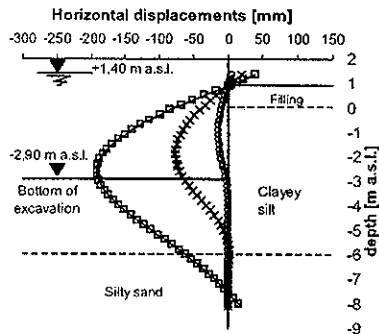
Figure 4. Calculated displacement of the "berlinese" piles
